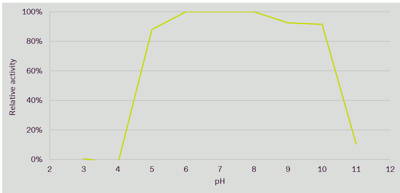
Fig. 3. Effect of pH on Neutrase® stability
